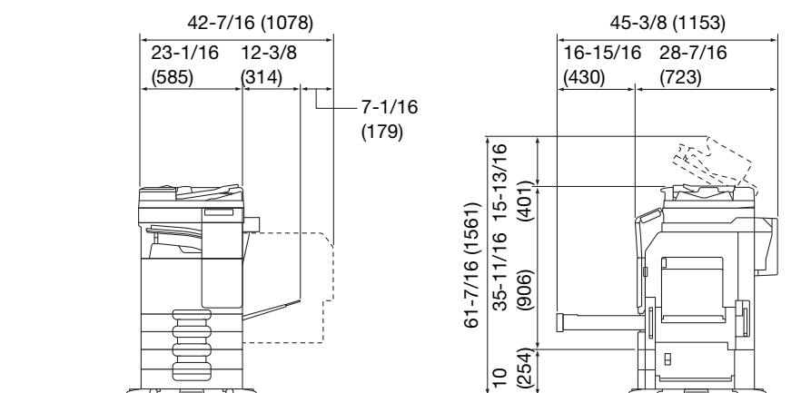
ineo+ 287/227 + DF-628 + PC-214 + MK-603 + JS-506
