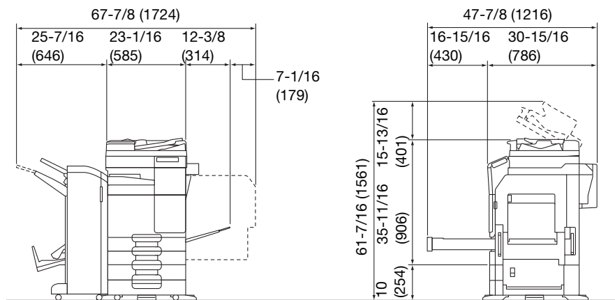
ineo+ 287/227 + DF-628 + PC-214 + MK-603 + RU-514 + FS-534 SD + MK-748 + CU-101
